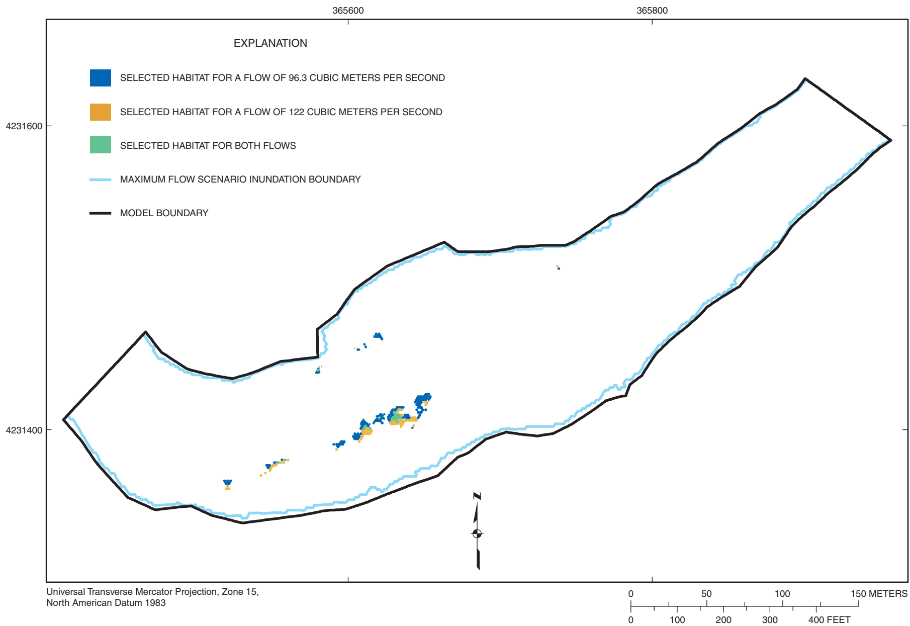
Figure 4-67. Selected habitat area distribution for habitat categories 16, 17 combined (channel catfish) at flows of 96.3 and 122 cubic meters per second at Marais des Cygnes River site MDC2.
